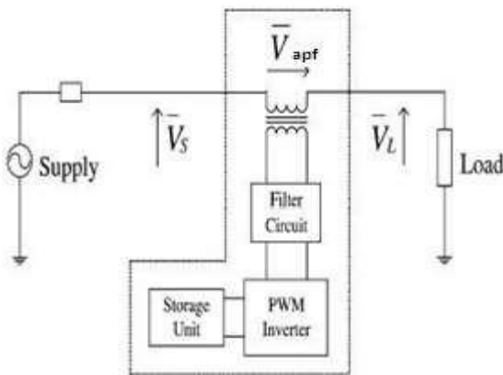
Fig1- Schematic diagram of Shunt activepower filter
