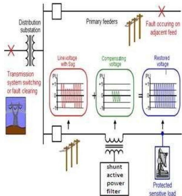
Fig2-Working principles of SAPF
