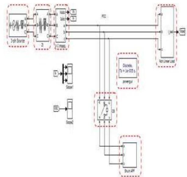
Fig 3: Simulink Model
