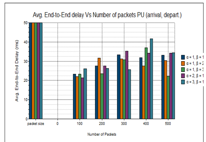
Fig. 2: Avg. End-to-End delay Vs number of packets
