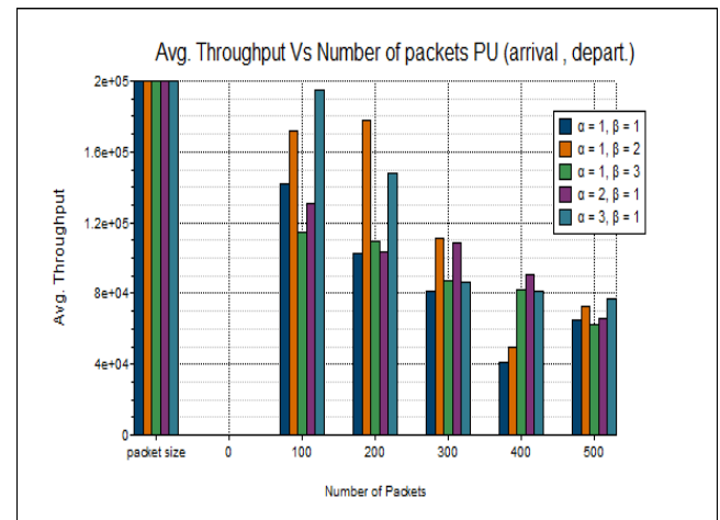
Fig. 1: Avg. Throughput Vs Number of packets (PU arrival and PU departure)
