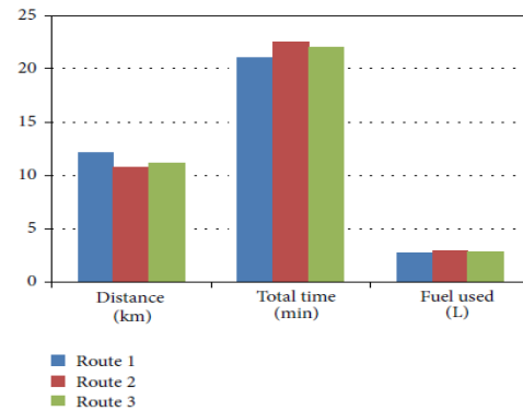
Figure5- Bargraphforthedistance,totaltraveltimes,andfuelused in moderatecongestion.
