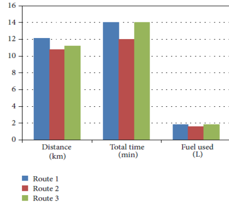
Figure4. Bargraphforthedistance,totaltraveltimes,andfuel used in free flow condition.
