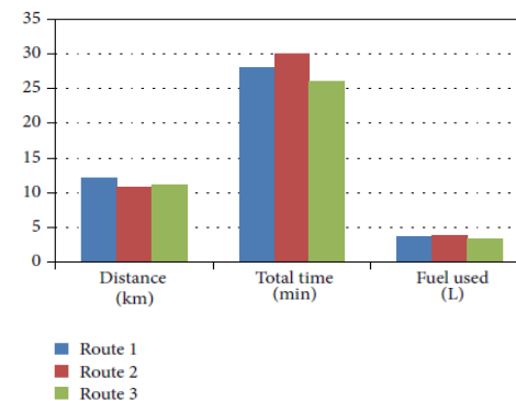
Figure6. Bargraphforthedistance,totaltraveltimes,andfuel used in congested condition.
