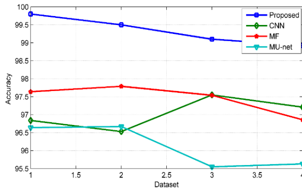
Figure: 4 Comparative result analysis of accuracy of DRIVE dataset employed proposed method, CNN, MF, and MU-net.
