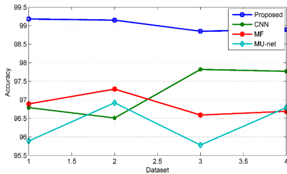
Figure: 8 Comparative result analysis of accuracy of STARE dataset employed proposed method, CNN, MF, and MU-net.
