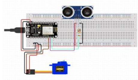
Fig 3.1-Circuit Diagram
