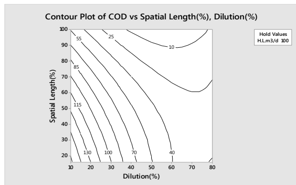
Fig.5 Contour plot showing effect of two independent variables (Hydraulic loading (m 3 /d) was held at their respective (centre level)
