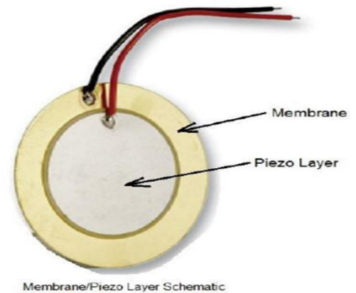
Figure 3: Piezoelectric Material
