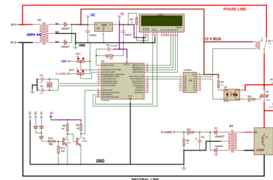
Fig 2: Circuit Diagram of Voltage Stabilizer.
