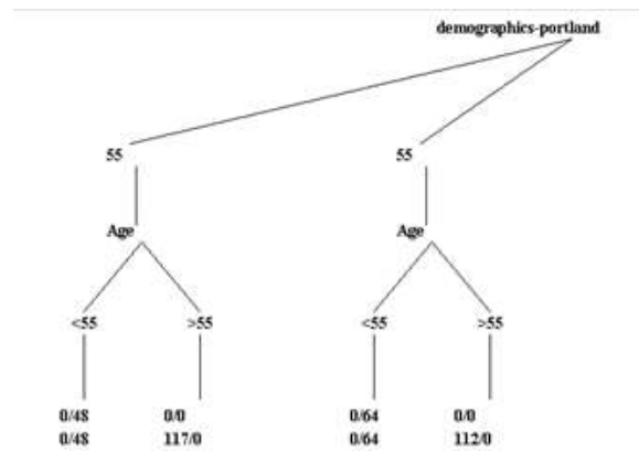
Fig.4: Decision Tree Generated
