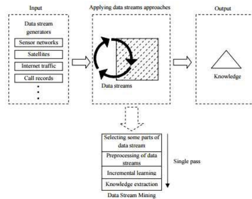
Fig.1: Proposed Architecture
