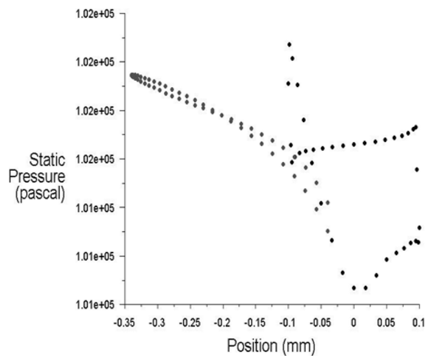
Graph-1: Pressure vs. position of blade
