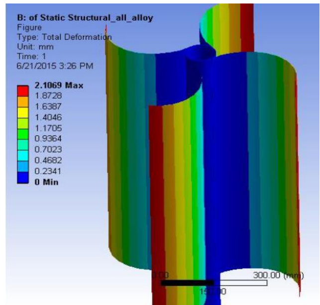
Fig-5: Deformation in Savonius turbine blades
