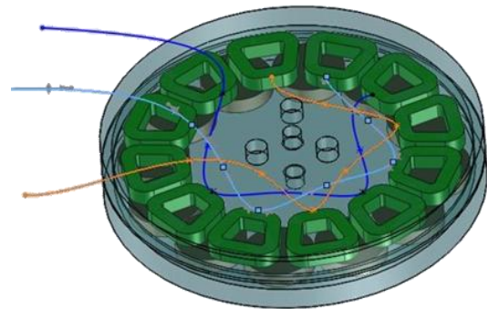
Fig -1: 3 phase connection of 12 coils
