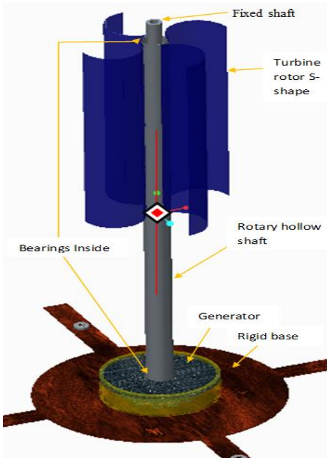
Fig-3: Savonius Vertical axis wind turbine
