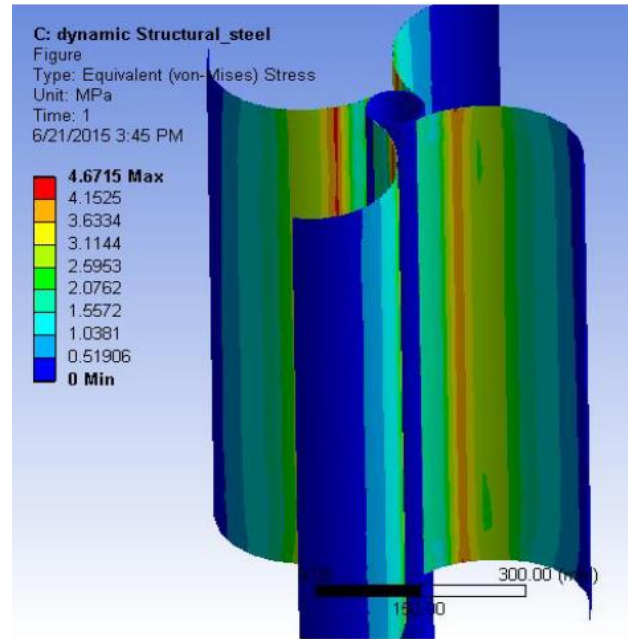
Fig-9: Equivalent stress in blades
