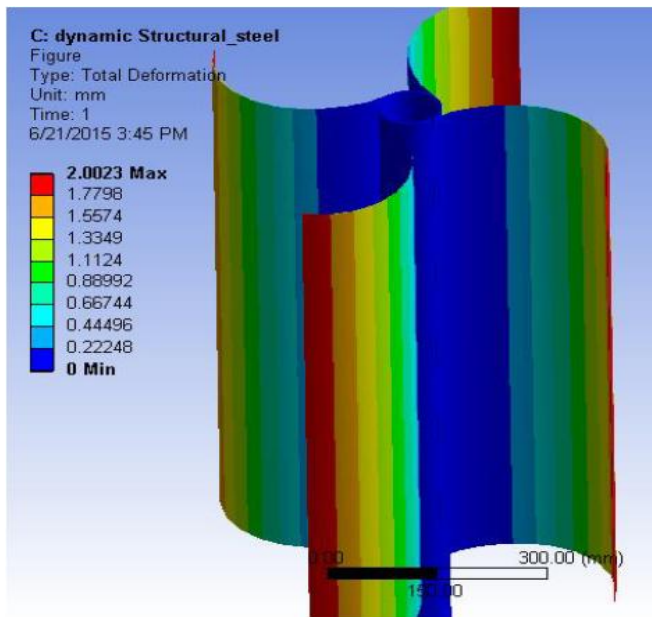
Fig-8: Total Deformation in blades
