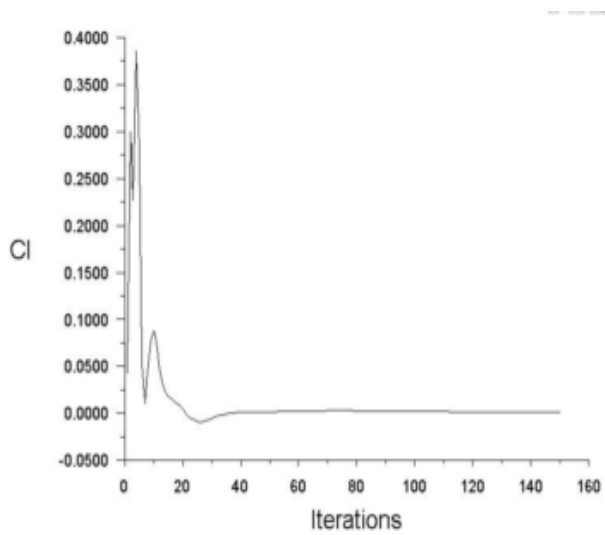
Graph-2: Co-efficient of lift vs. No. of Iterations
