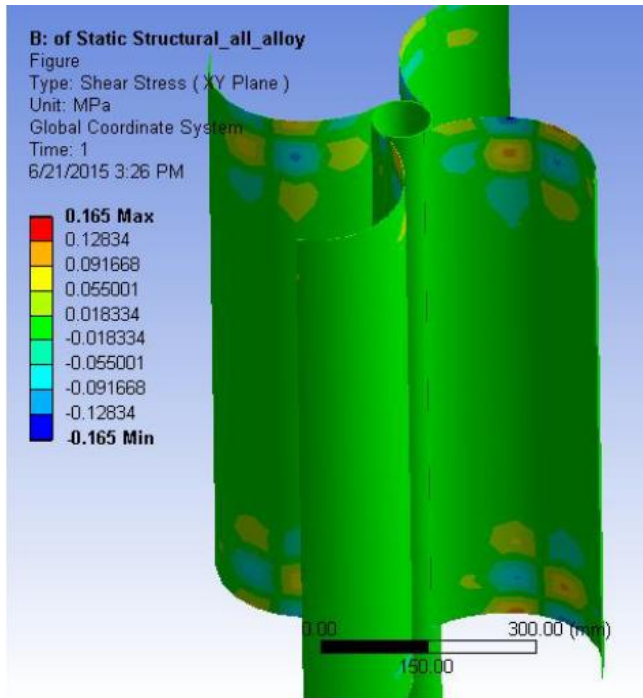
Fig-7: Shear stress on XY plane in Savonius blades
