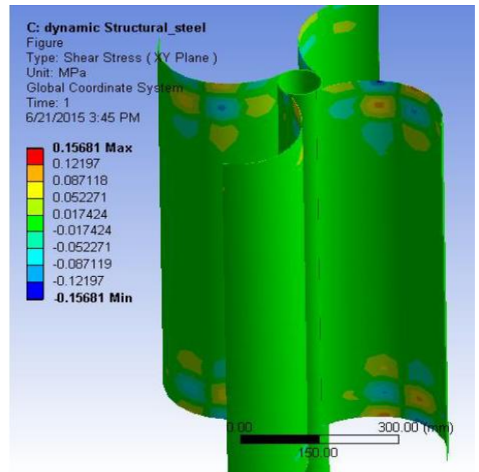
Fig-10: Shear stress on XY plane in blades
