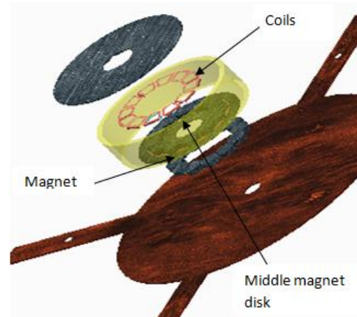
Fig-2: Expanded view of multi stage generator
