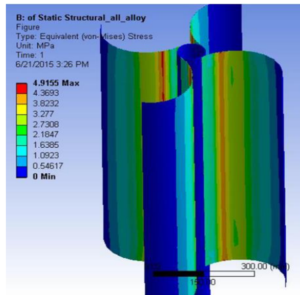
Fig-6: Equivalent Stress in Savonius turbine blades
