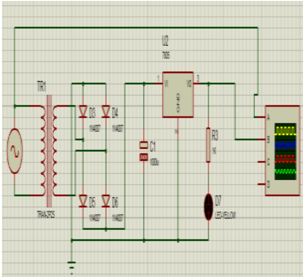
Fig 4- Circuit diagram for Power supply
