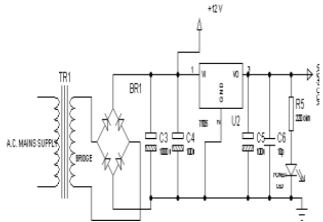
Fig 3 of circuit diagram of power supply circuit Component of power supply circuit
