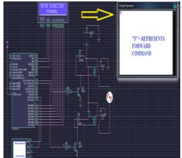
Fig 6.-Output for forward direction
