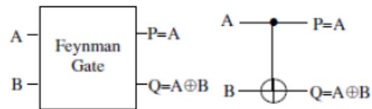
Figure 2.1: Feynman Gate
