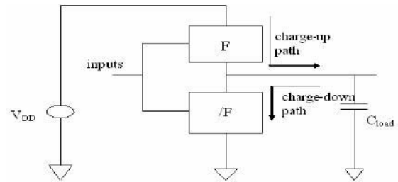
Figure 1. Charging and Discharging in Conventional System
