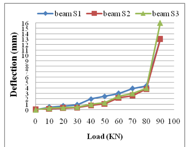
Figure 4. Relationship between load and deflection of beam S1, S2, S3
