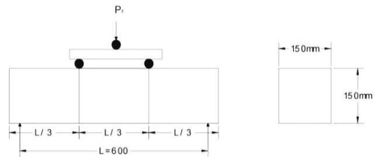
Fig. 2- fig shows two point loading setup
