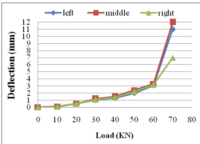
Figure 1. Relationship between load and deflection of beam S1
