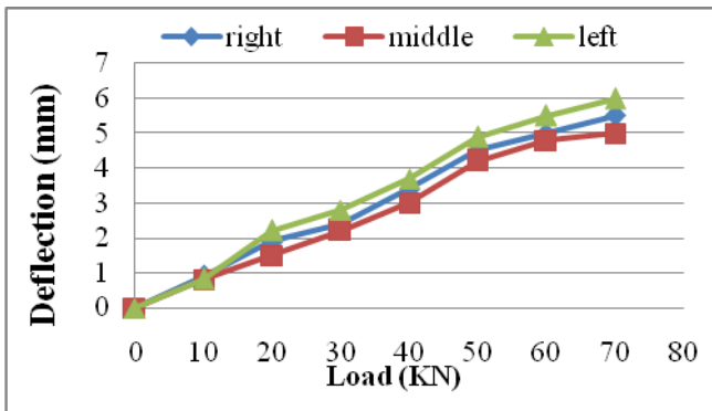
Figure 1. Relationship between load and deflection of beam S1
