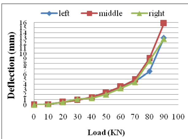
Figure 2. Relationship between load and deflection of beam S2
