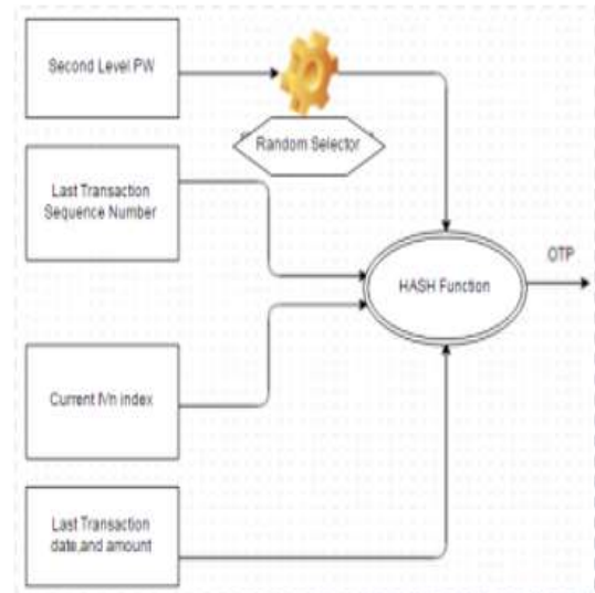
Fig.5 OTP generator
