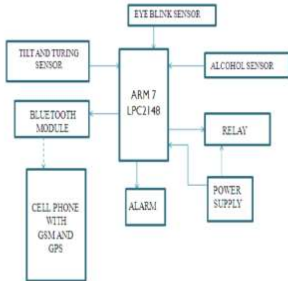
Figure4:Block Diagram
