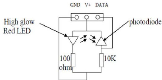
Fig.9- Analog optical Sensor
