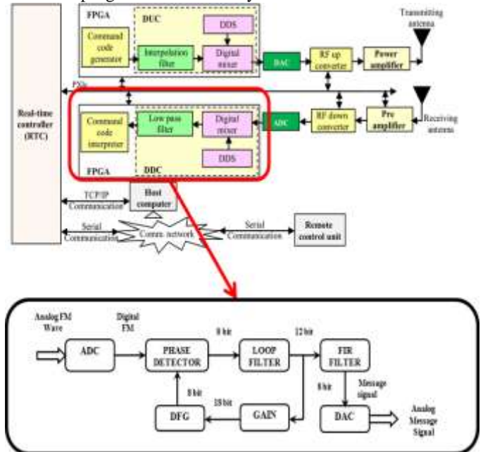
Fig(2). DPLL Architecture
