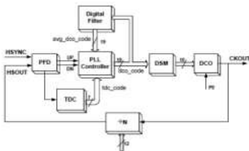
Fig(1). Block Diagram of DPLL
