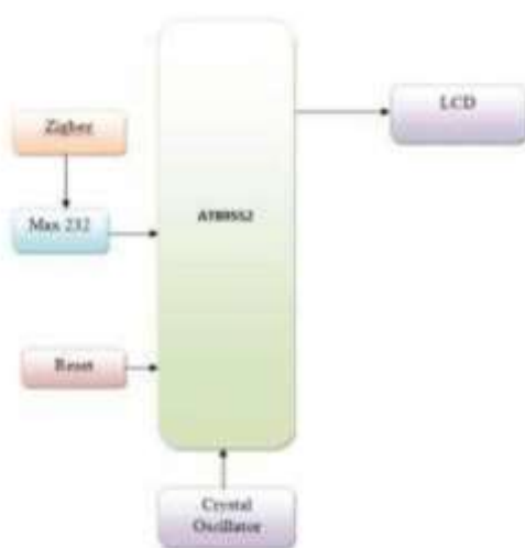
fig 2.receiver
