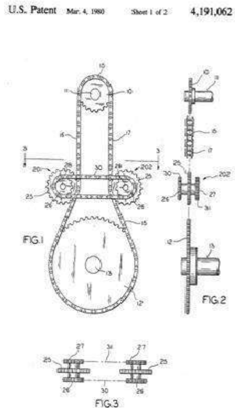
Fig. 4- fig shows the Chain drive & Automatic chain tensioner unit.
