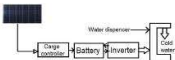
Fig.3 Solar powerd water cooling systel
