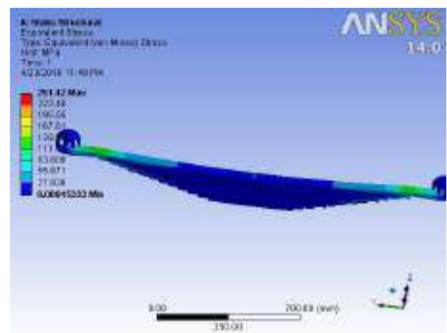
Fig. 4- Rear spring
