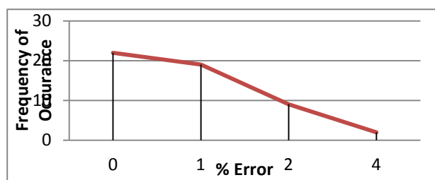
Fig. 5- % Error Frequency graph for % of Carbon Equivalent: II01
