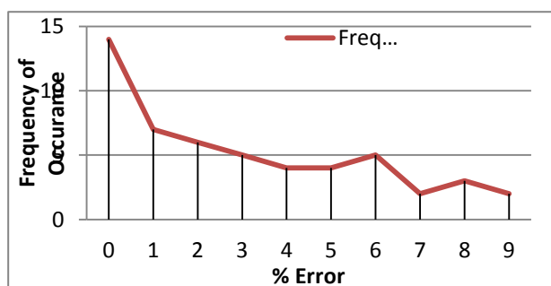
Fig. 13- % Error Frequency graph for Number of Actual Charging required : Π010
