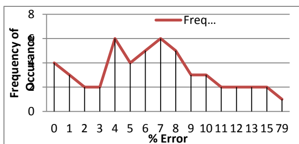
Fig. 14- % Error Frequency graph for Strength of Material : Π011
