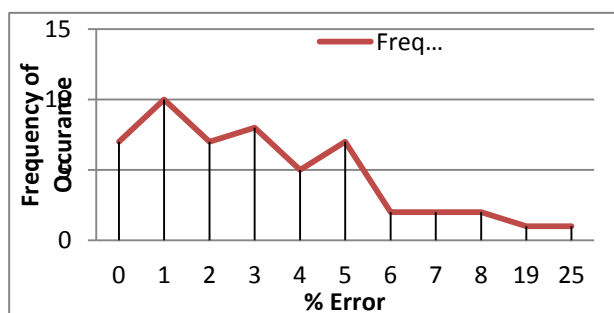
Fig. 14- % Error Frequency graph for Strength of Material : Π011
