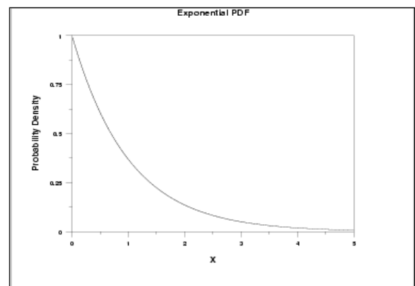
Fig. 3- Probability density function exponential distribution
