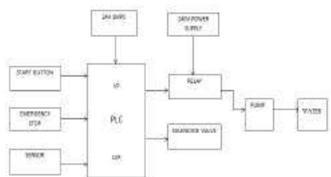
Fig. Block diagram of Automatic car washing using PLC
