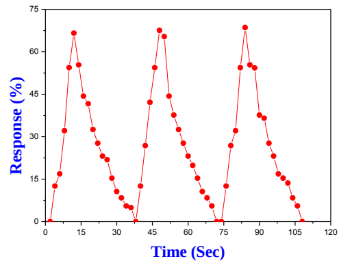
Fig. 6: Response and Recovery curve for nano ZnO at operating temperature 300^\circ C to 2500 ppm of H_2S
