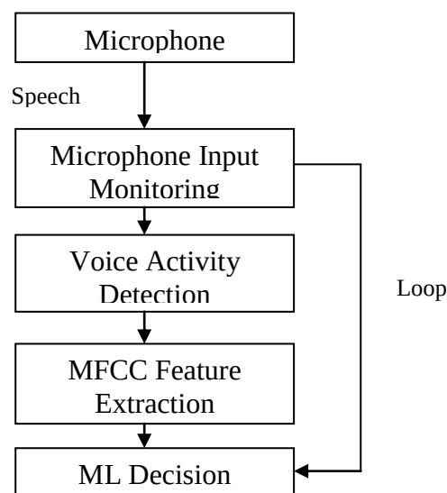
Fig. 1 Block diagram of the Voice Recognition
