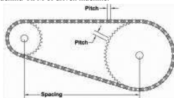
Fig. 1- fig shows the Chain drive mechanism in cycles But in case of cycles,
