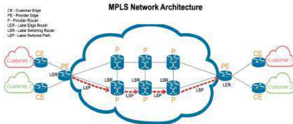
Figure 1: MPLS Architecture
