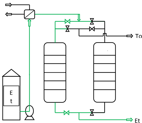
Figure.1 Symbolic Diagram of Molecular Sieve Dehydration
