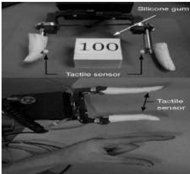
Fig 2 . Tactile sensor
