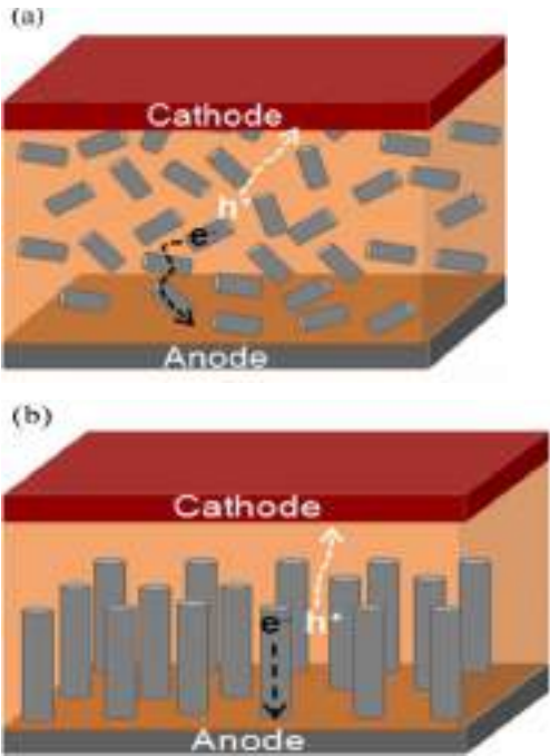
Fig. 1. Demonstration of two different constructions of polymer solar cells. (a) BHJ solar cell. (b) Nanostructured solar cell. Carrier transport paths were indicated by dashed arrows. Hole transport through polymer phase and electron hop through TiO 2 network pathways in BHJs or directly pass along ZnO nanorods in nanostructured solar cells.
