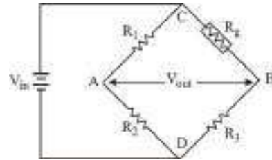
Fig 2-Wheatstone bridge circuit
