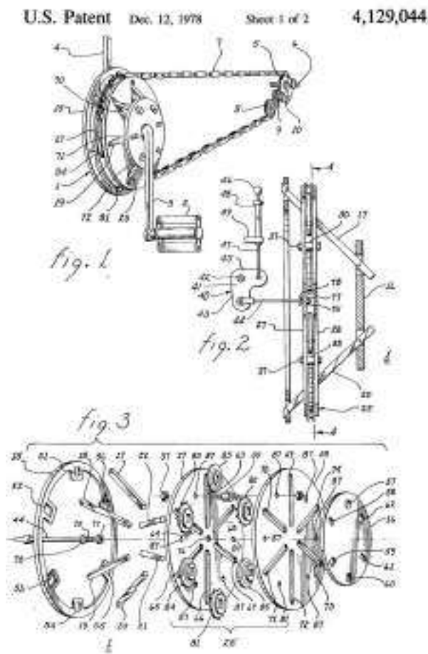
Fig. 3- fig shows the Variable gear ratios chain drive system.
