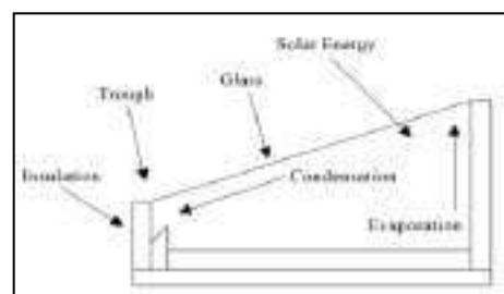
Fig.1-Simple solar still
