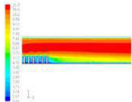
Figure 21 Velocity Plot for Deep Pin Fin
