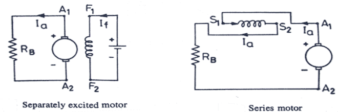
Fig1. Dynamic braking
