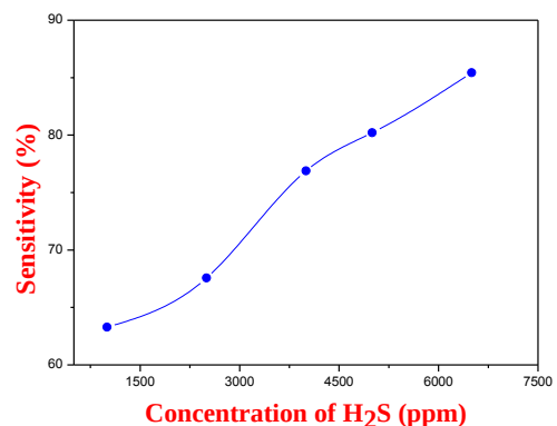
Fig. 7: Dependence of response of nano ZnO on H_2S concentration at operating temperature of 300^\circ C
