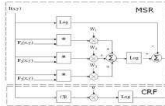
Fig.1 Block Diagram for MSRCR Algorithm
