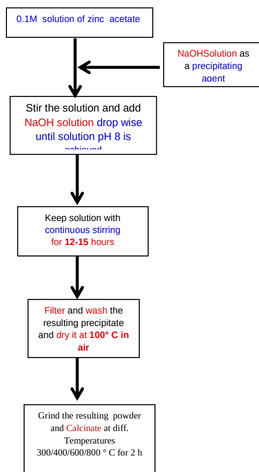
Fig. 1 : A schematic diagram of the synthesis procedure.
