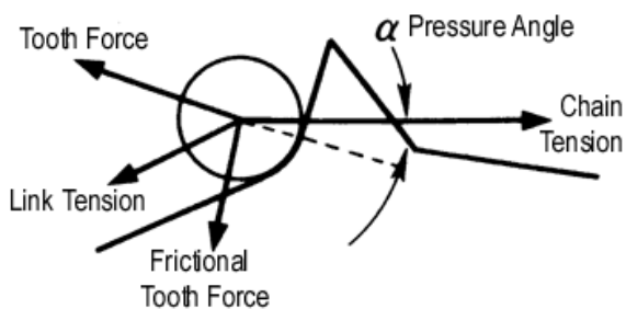
Fig: The balance of forces around the roller
