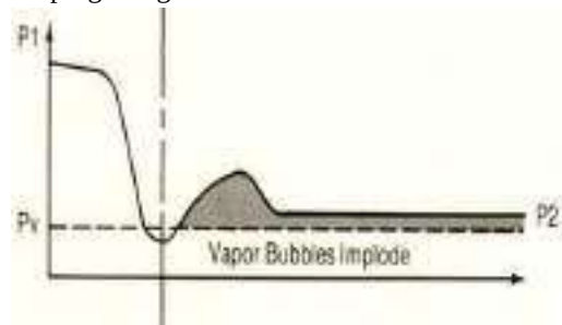
Figure 4 Cavitation in Control valve
