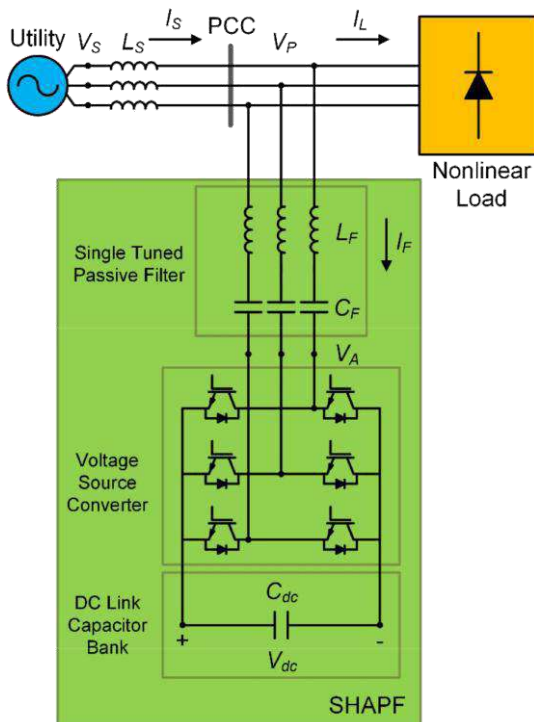
Fig. 1- fig shows the Power circuit Configuration
