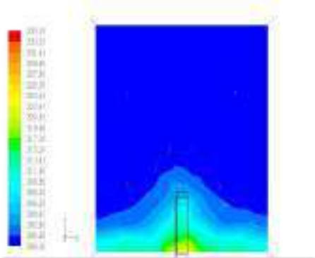
Figure 19 Temperature Contours of rectangular fin at plot Z=38 mm
