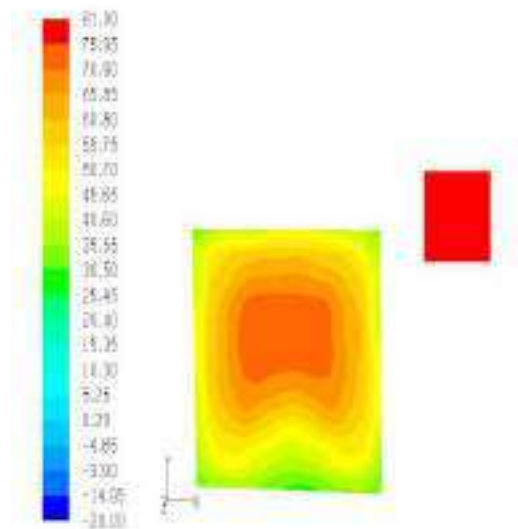
Figure 23 Total Pressure Plot for Cyl Pin Fin
