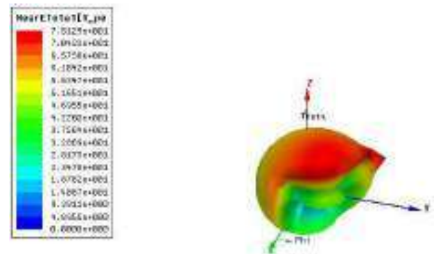
Fig. 8- near E-total on FR4 for double step feed line circular patch antenna
