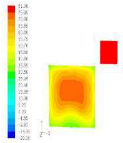
Figure 24 Total Pressure Plot for Drop-Shaped Pin Fin
