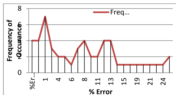
Fig. 11- % Error Frequency graph for Cast Iron Scrap Outlet: II08
