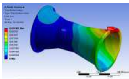
Fig. Deformation of rim
