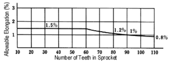
Fig.2.11: Elongation versus the number of sprocket teeth
