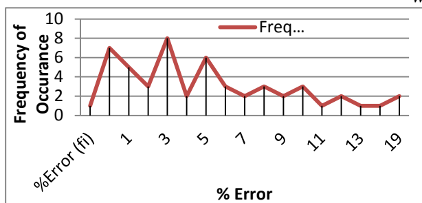
Fig. 12- % Error Frequency graph for Waste In front of Cupola : Π09
