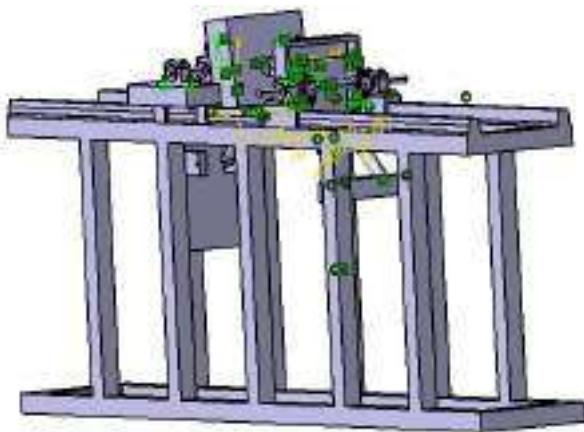
Fig1:- Design of hydraulic mold splitter and tipper equipment
