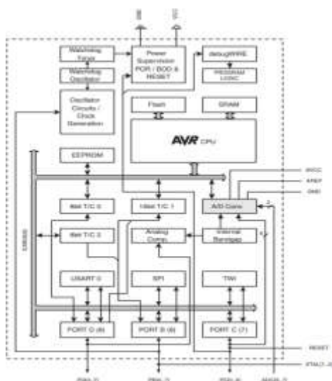
Fig.5. Block diagram of ATmega328 microcontroller.
