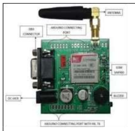
Fig .6.- Front view of a GSM/GPRS sim900A module
