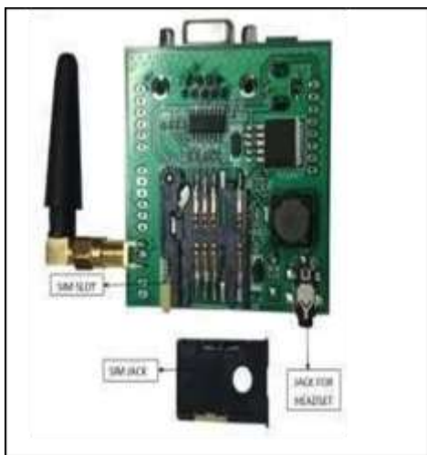
Fig.7. Rear view of GSM/GPRS module
