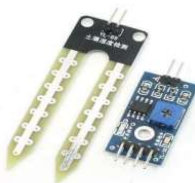
Fig 9: YL-69 moisture sensor.
